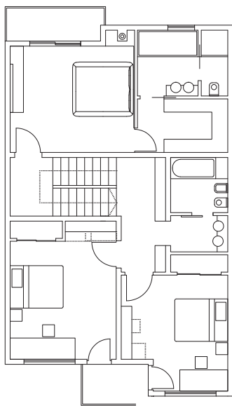
Plan etaj / Floor plan
